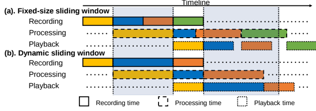
Fig. 1: Dynamic vs. fixed-size sliding windows. Different windows are indicated by different colors. Each window is processed by the network individually. The gray areas indicate the time period in which CPU cycles are occupied by other processes and thus the network processing time increases.
