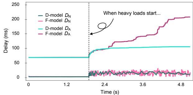
Fig. 3: Comparison of realtime performance between dynamic and fixed sliding window approaches. We artificially increase the network processing time randomly by 1-7 times after 2 seconds to simulate CPU power fluctuation. The curves are averaged results over 100 trials with a fixed random seed.
